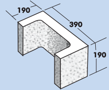
20.34 Pilaster 'C' Type
