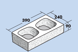
H25.04 Standard or Corner Half High
