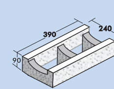
H25.14 Bond Beam Depressed Web
