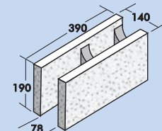
15.16 Open End Bond Beam
